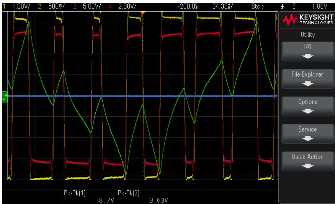
FIG. 2. Oscilloscope screen showing: voltage corresponding to the generated waveform in the arbitrary waveform generator (red), voltage across the calibrated resistor in the primary circuit (green), and the induced rectangular PWM voltage in the secondary coil (yellow).
